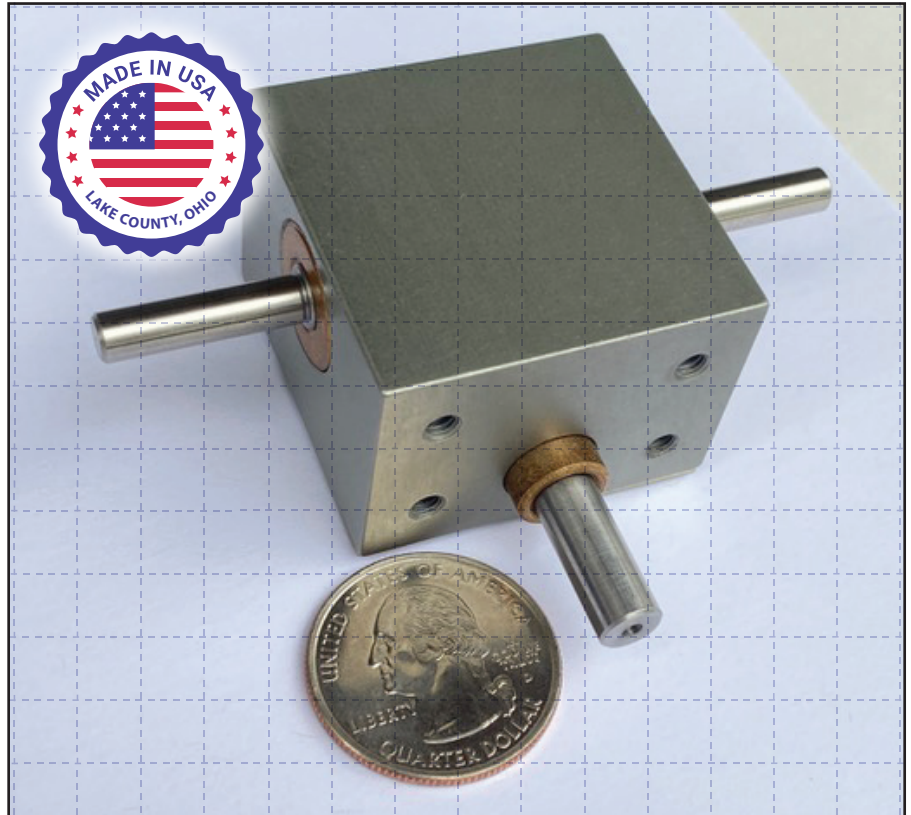
SW-3 / SW-4 Miniature Right Angle Gearbox
